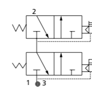
3/2 NC Connected Valve
