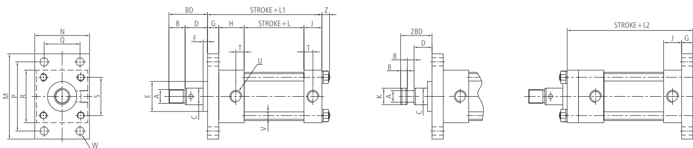
Front/Rear Flange
