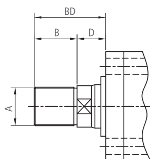
Male Thread
