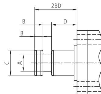
Coupler Type
